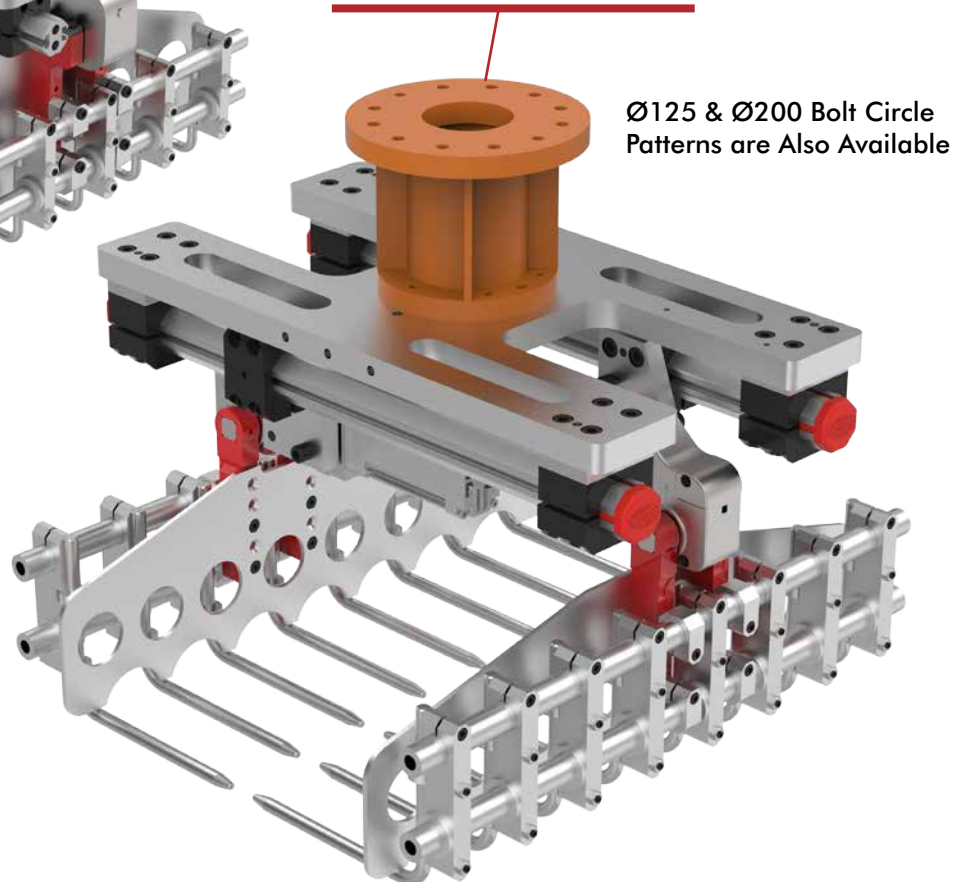
Robot Mount Stand-Off with \text{\O}160 Bolt Circle Pattern DBG100-2-S04-160BC-KIT
