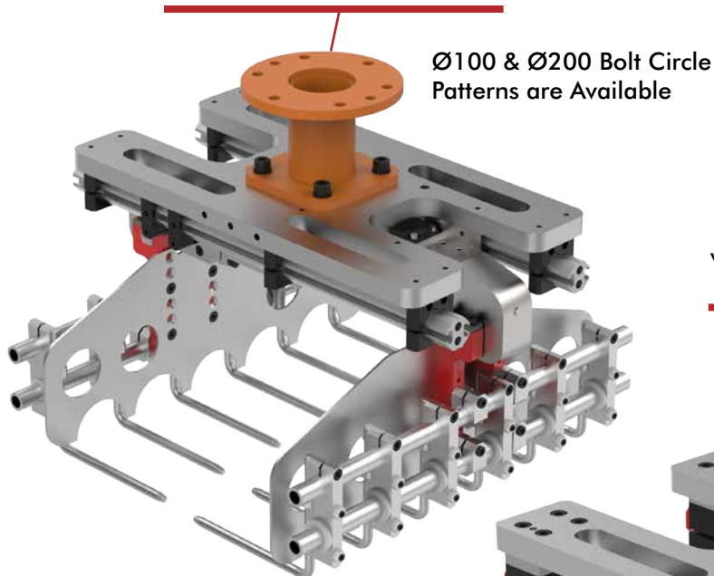
Robot Mount Stand-Off with \text{\O}125 Bolt Circle Pattern DBG50-2-S04-125BC-KIT
